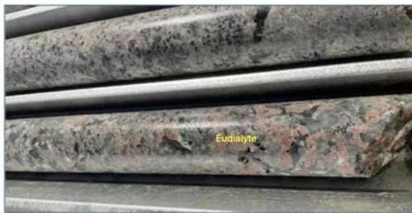
Coarse grained Eudialyte (pink) in drill core from the Tanbreez Hill area demonstrating the coarse nature of the mineralisation(assays are included in the MRE estimate.
