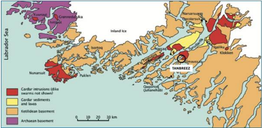
The Ilimaussaq Complex and Tanbreez location
