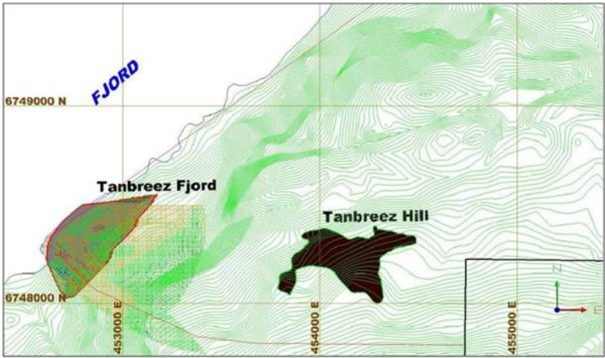
Tanbreez Hill and Tanbreez Fjord location map.
