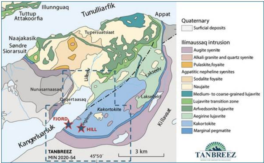
Kakortokite outcrop dominates the Tanbreez Area east of the Kangerluarsuk Fjord.
