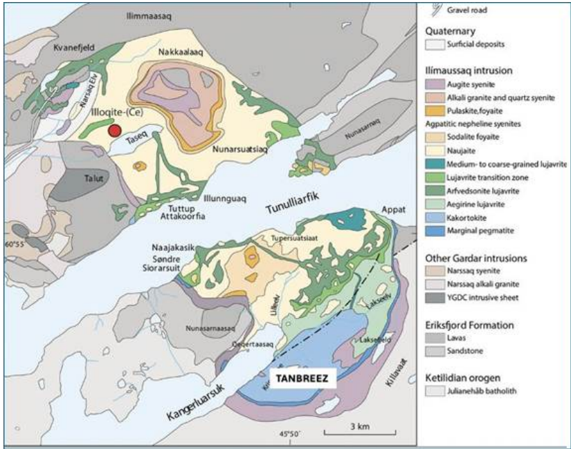
Geological setting of the Ilimaussaq complex.
