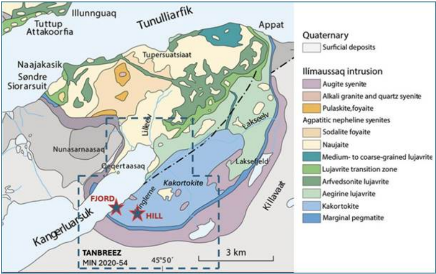
Kakortokite outcrop dominates the Tanbreez Area east of the Kangerluarsuk Fjord. Tanbreez Hill and tanbreez Fjord deposits shown within kakortokite
